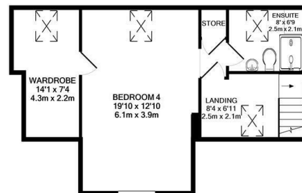
2ND FLOOR
