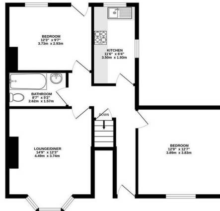
GROUND FLOOR 650 sq.ft. (60.4 sq.m.) approx.
