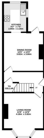
GROUND FLOOR 442 sq.ft. (52.1 sq.m.) approx.
